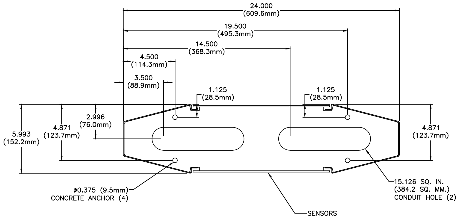
BE800-S / BE800-W FOOTPRINT 1/1/14
