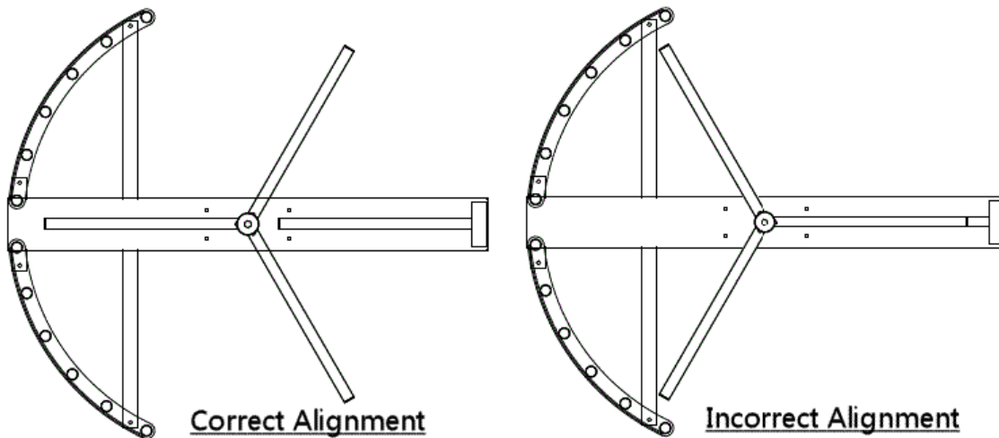
Figure J: Correct rotor alignment (left) vs. incorrect rotor alignment (right).
