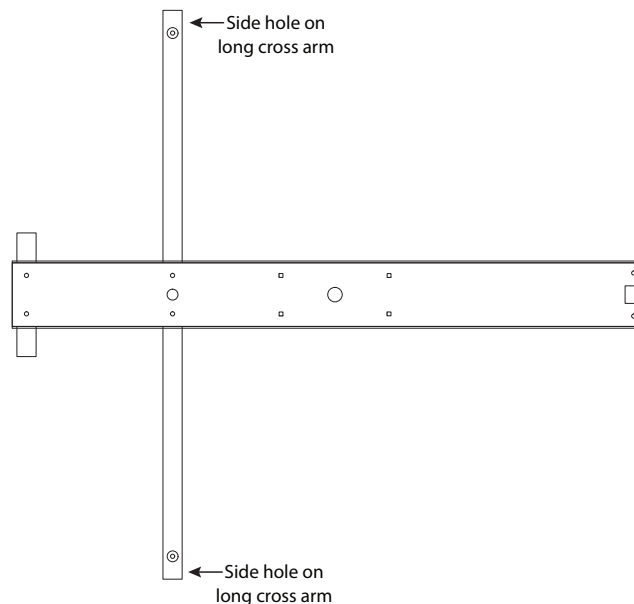
Upper View
