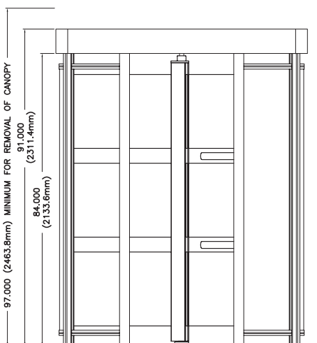
P60 with optional T36-ADA door
