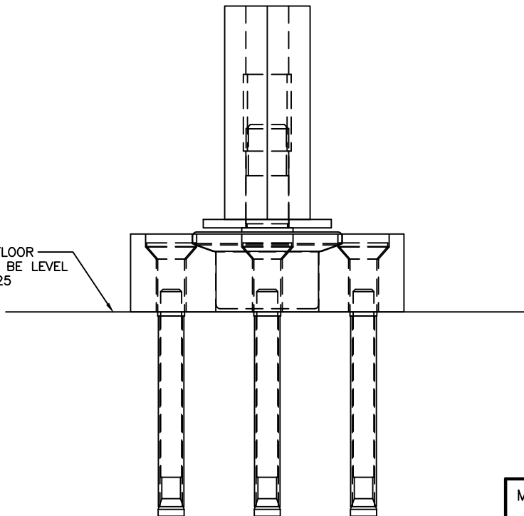
ASSEMBLY ELEVATION VIEW
