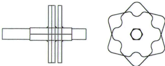
CA-6059 ANTI-BACKUP CAM ASSEMBLY
